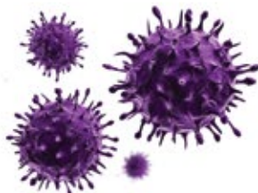
Spores
